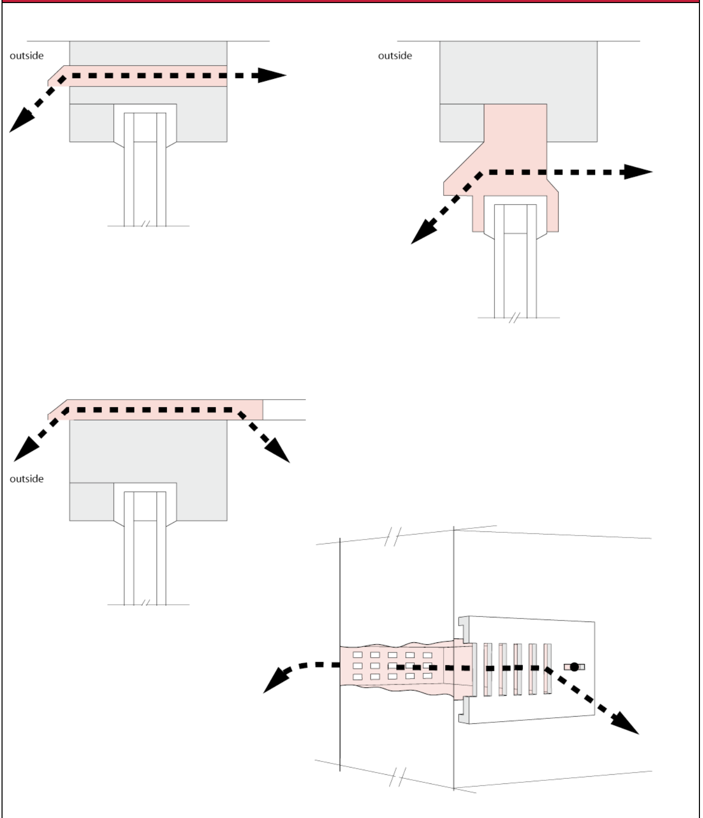
Diagram 1.1 Provision for background ventilation
