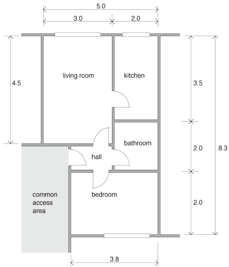
Diagram C1 Ground floor flat plan
