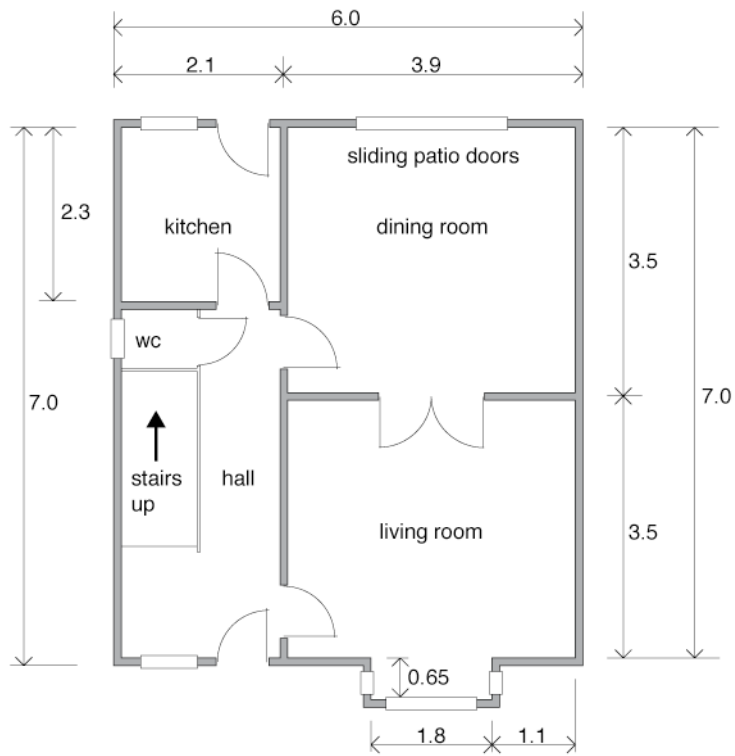
Diagram C2 Semi detached house ground floor plan
