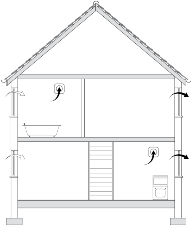
Background ventilators and intermittent extract fans
