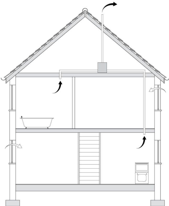
Continuous mechanical extract
