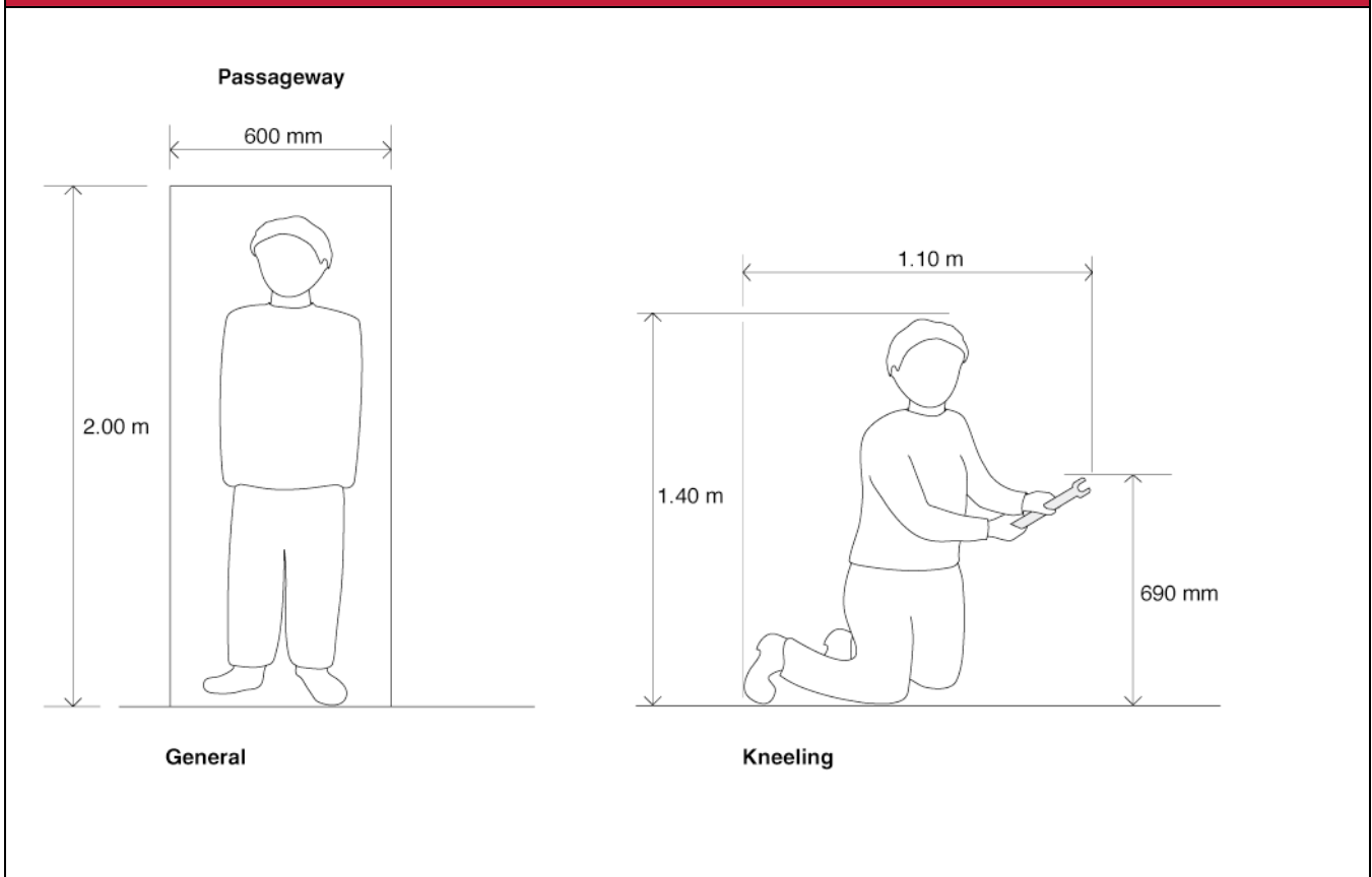
Diagram 3.1 Space for access
