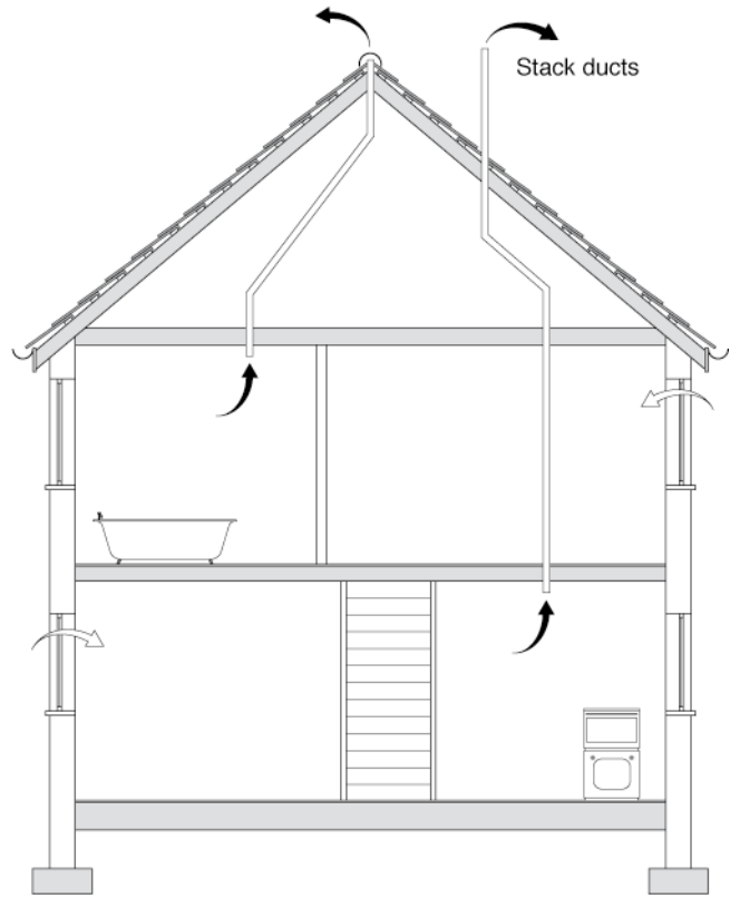
Passive stack ventilation
