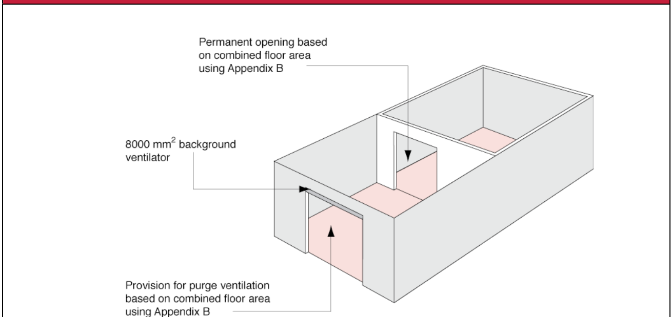
Diagram 2.3 Two habitable rooms treated as a single room for ventilation purposes
