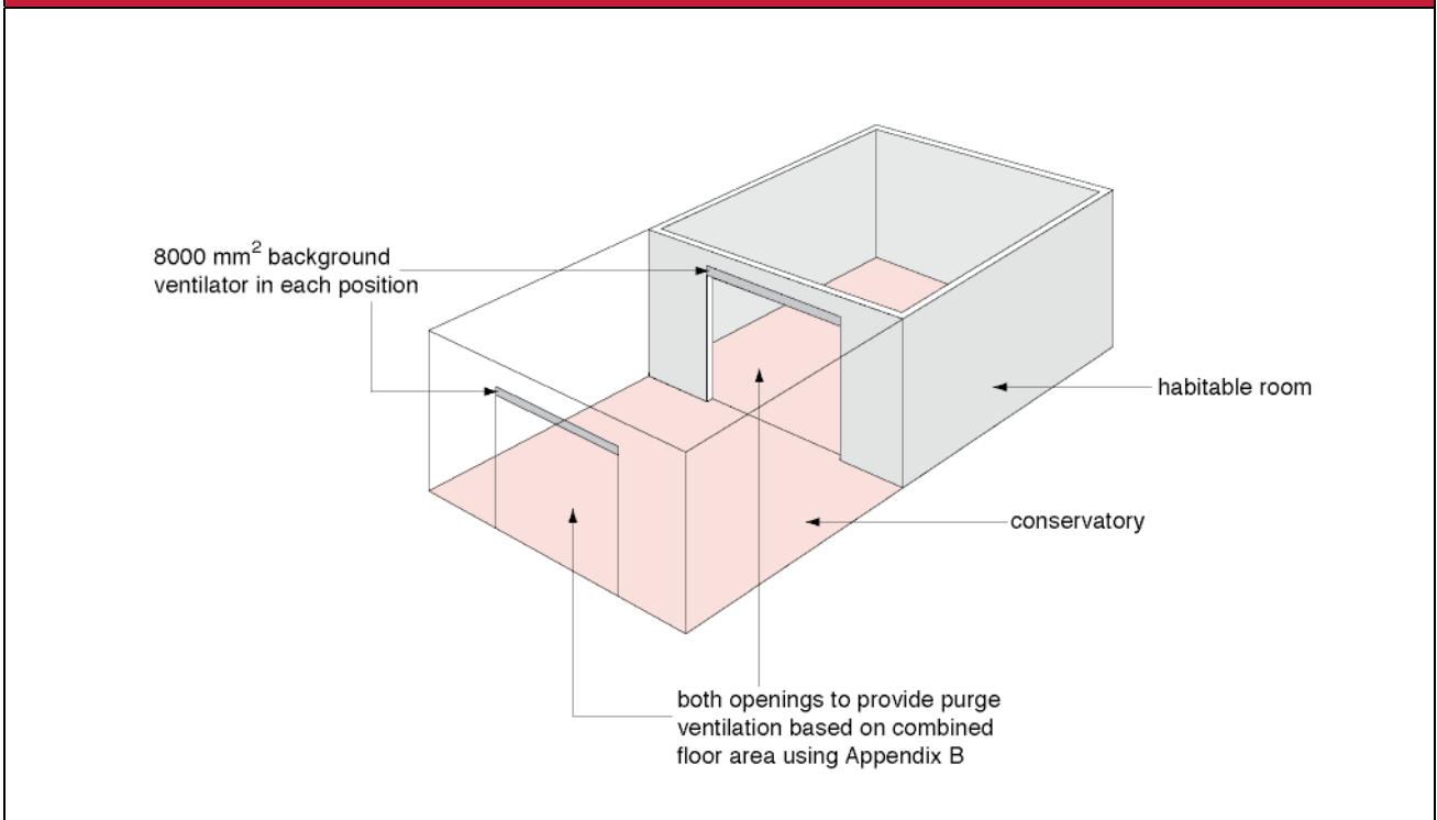
Diagram 2.4: A habitable room ventilated through a conservatory
